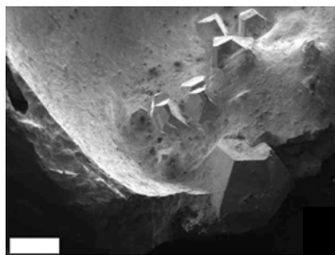
Fig. 25. SEM image of moissanite (SiC) crystals in iron silicide matrix. Scale bar 1 mm
