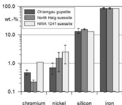
Fig. 24. Comparison of analyses of Chiemgau gupeite and meteoritic suessite. Suessite data from [46] and [89]
